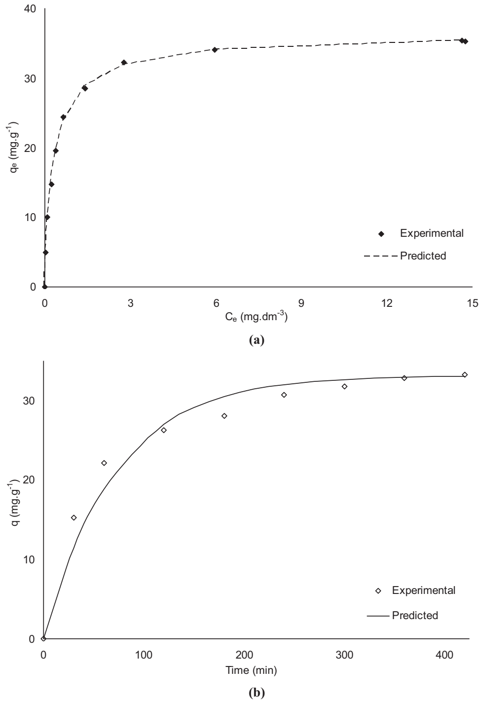
Fig. 4. (a) Langmuir–Freundlich adsorption isotherm of methylene blue on biochar. (b) Adsorption kinetics of methylene blue on biochar.
