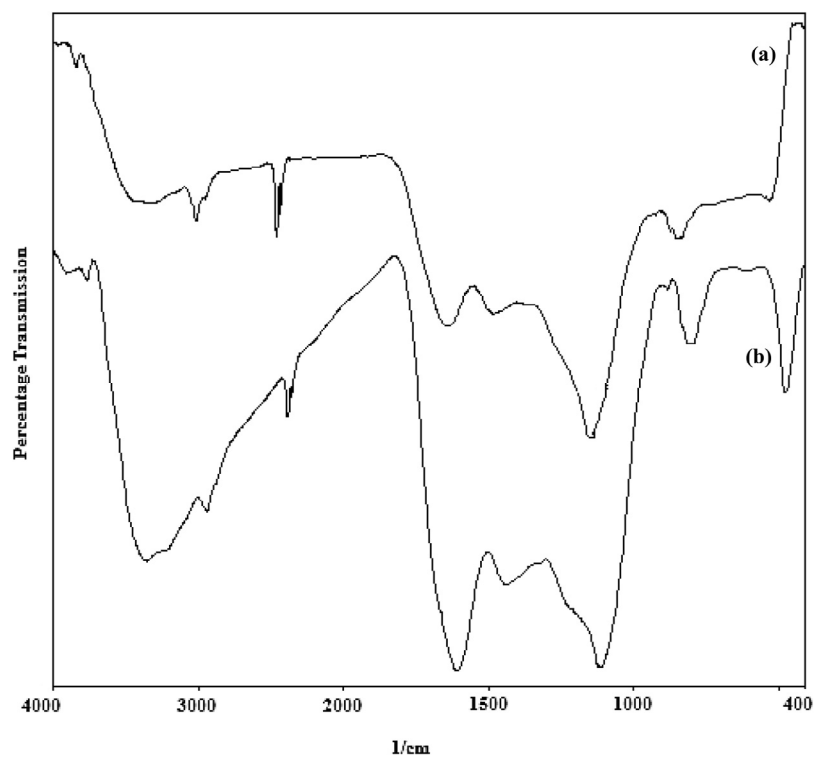
Fig. 1. FTIR spectra for (a) BAB before adsorption and (b) BAB after adsorption.
