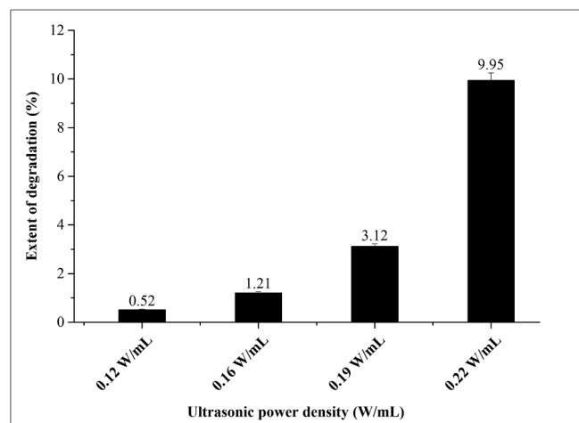
Fig. 3. Effect of ultrasonic power density on the percentage degradation of thiamethoxam (Operating conditions: volume = 250 mL, pH = 2.0, temperature = 30 \pm 2 °C, initial concentration of thiamethoxam = 20 ppm).
