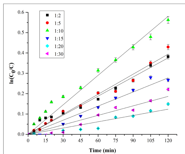
Fig. 6. Kinetics of ultrasonic degradation of thiamethoxam at different molar ratio of thiamethoxam: \text{H}_2\text{O}_2 (Operating conditions: volume = 250 mL, initial concentration of thiamethoxam = 10 ppm, pH = 2.0, temperature = 30 \pm 2 °C and amplitude = 100%).
