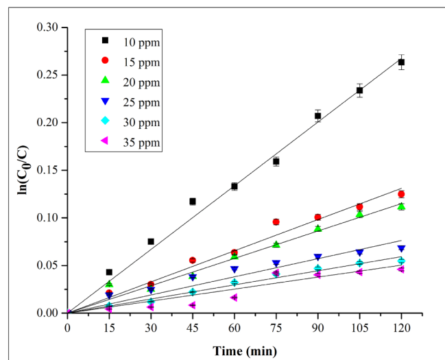
Fig. 4. Kinetics of ultrasonic degradation of thiamethoxam at different initial concentrations of thiamethoxam (Operating conditions: volume = 250 mL, pH = 2.0, temperature = 30 \pm 2 °C and amplitude = 100%).
