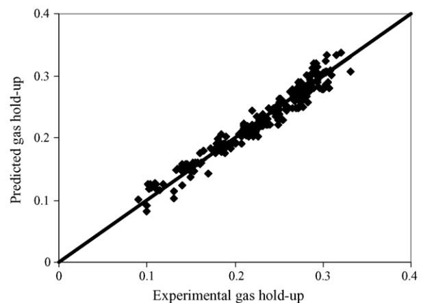
Fig. 3. Comparison of predicted gas hold-up with experimental.
