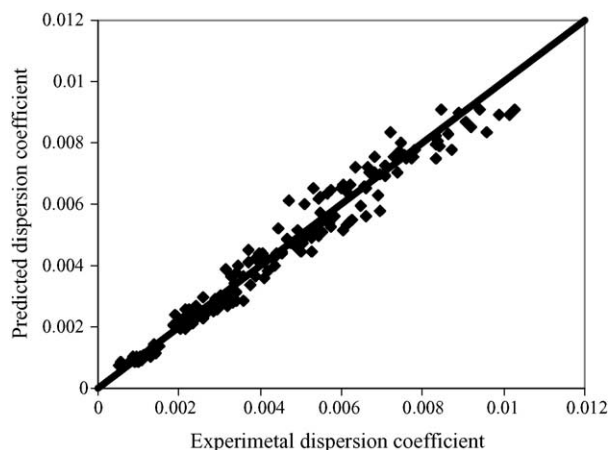
Fig. 10. Parity plot for dispersion coefficient.
