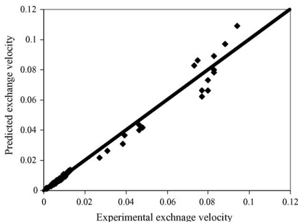
Fig. 11. Parity plot for intercell exchange velocity.
