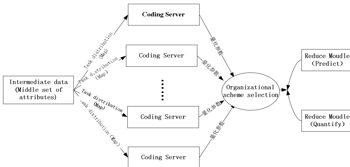
Figure 2. The Generative Process of Middle Data
