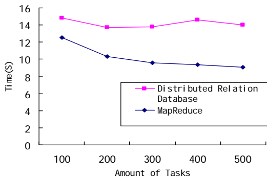
Figure 4 Work Efficiency Test Result
