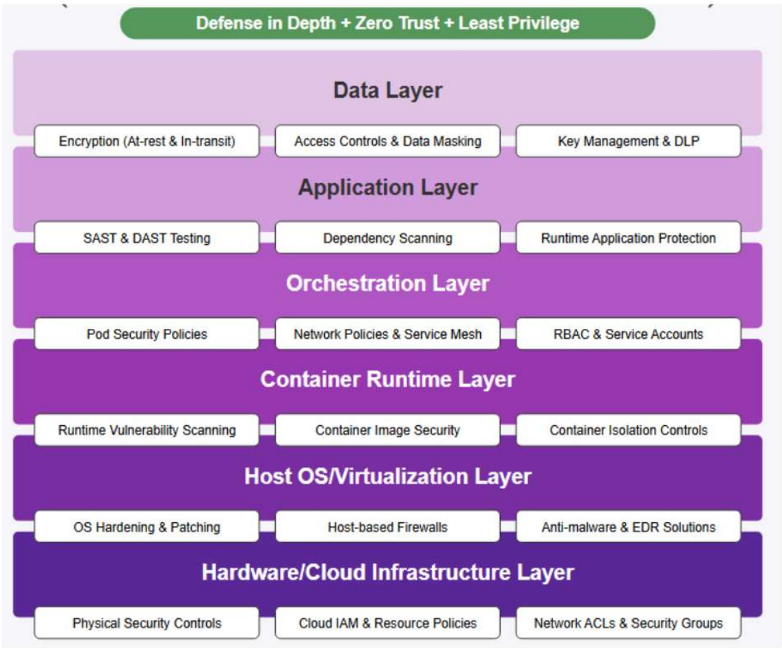
Figure 3 illustrates the security measures applied at different layers of the cloud-native infrastructure stack.
