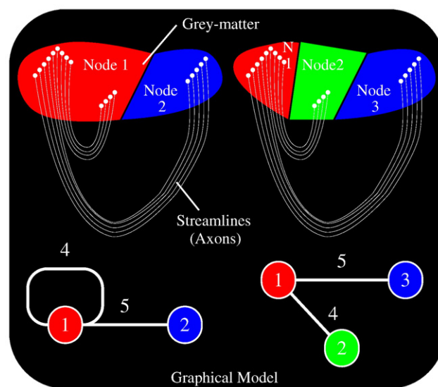
Fig. 1. Example parcellation of a forking U-fiber. The leftmost parcellation is too coarse and fails to characterize the left branch of the fork. In a graphical model, the left branch manifests as a self-loop about node 1. The rightmost parcellation is however fine enough to characterize both branches. The weight assigned to each link corresponds to the total number of intersecting streamlines.
