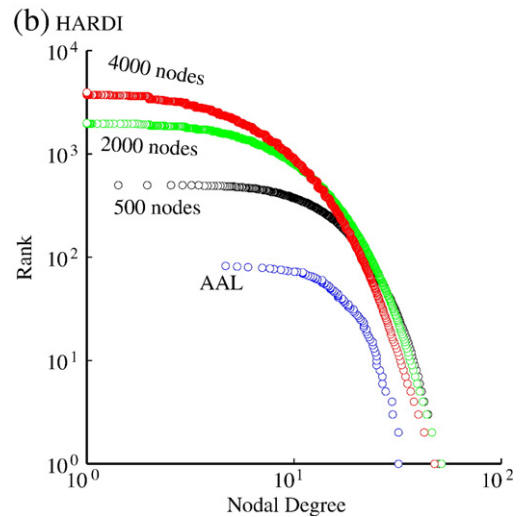
Fig. 8. Nodal rank plotted as a function of degree for DTI and HARDI. For each of 100 random parcellations, a brain network was constructed and its degree sequence ranked such that the node with largest degree was assigned a rank of one. For each rank, the mean of the corresponding nodal degree was computed across the 100 networks. This process was repeated for the three acquisitions. Therefore, a total of 100 \times 3 = 300 networks were ranked. Rank-degree plots were then constructed based on the average across these three acquisitions.
