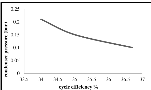
Figure 3 variation of cycle efficiency with condenser pressure
