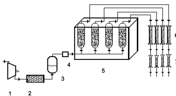
Fig. 1. Schematic set-up of column bioreactor system. 1 air pump, 2 air filter, 3 air moisturizing unit, 4 air distributor, 5 columns in water bath, 6 \text{CaCl}_2 columns, 7 adsorbent columns
