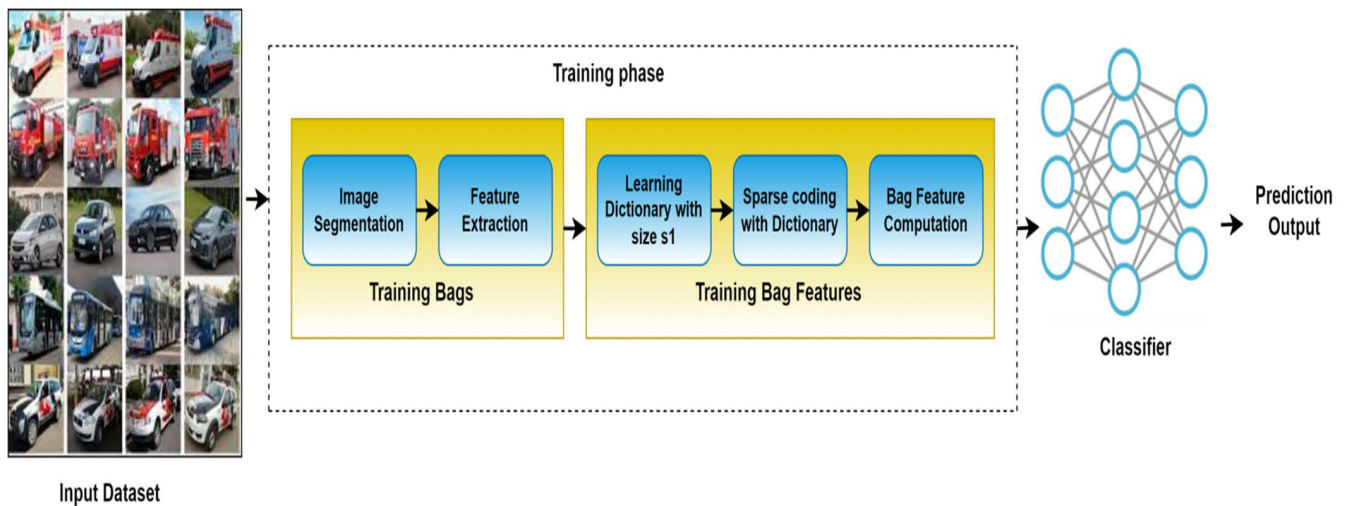
FIGURE 8. Framework of multiple instance learning.
