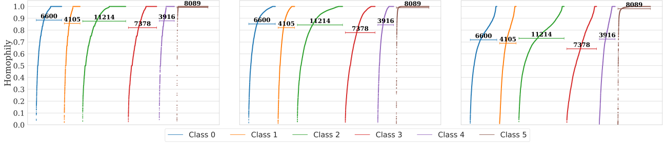
Figure 10: Node Homophily Distribution Scores for DBLP-CA.
