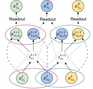
Figure 3: MultiSet layout.
