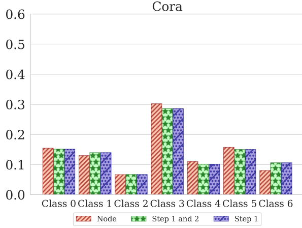
(a) Class distribution for Cora.
