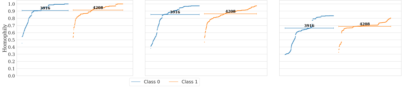
Figure 13: Node Homophily Distribution Scores for Mushroom.
