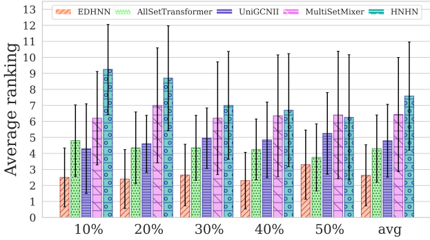
Figure 4: Average rankings and standard deviations at different training percentages, with overall average performance.
