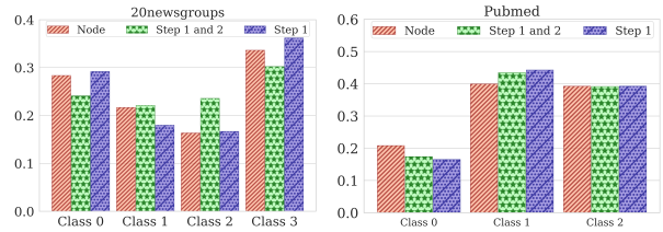
Figure 6: Class distribution shift induced by mini-batching: ‘Node’ represents the original node class distribution, ‘Step 1 and 2’ the resulting one after sampling both hyperedges and nodes, and ‘Step 1’ when only sampling hyperedges.
