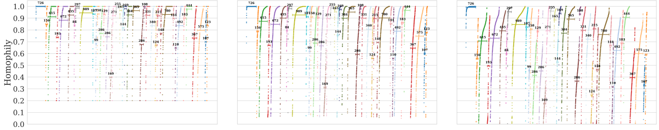
Figure 12: Node Homophily Distribution Scores for ModelNet40.
