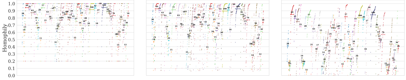
Figure 11: Node Homophily Distribution Scores for NTU2012.
