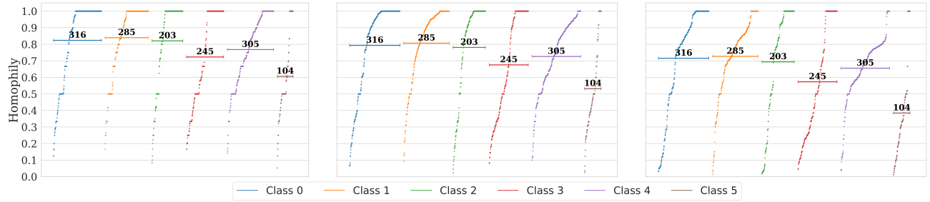
Figure 8: Node Homophily Distribution Scores for Citeseer.
