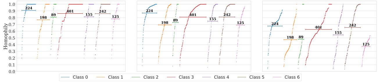
Figure 7: Node Homophily Distribution Scores for Cora.
