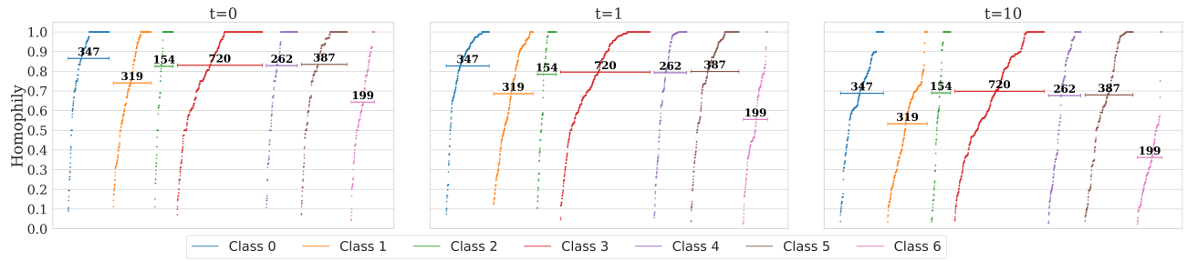
Figure 9: Node Homophily Distribution Scores for CORA-CA.
