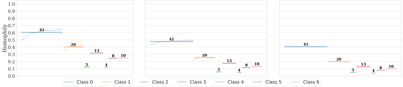
Figure 15: Node Homophily Distribution Scores for ZOO.
