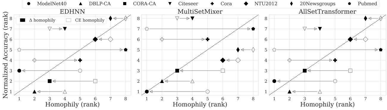
Figure 5: Joint visualization of rank dependencies, showing Norm. Acc. versus \Delta Homophily (Eq. 4 at step t = 1 and \mu = 0.1 ) and CE Homophily (Wang et al., 2023). Norm. Acc. (Eq. 14) is assessed for various instances of model A (specified in column titles), with model B being MLP CB. Both axes represent rank values, with lower values indicating better metrics. Arrows denote the rank shift in homophily between CE homophily and \Delta homophily for each dataset.
