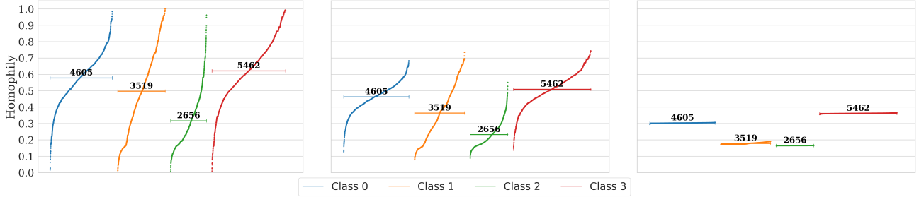
Figure 14: Node Homophily Distribution Scores for 20NewsW100.
