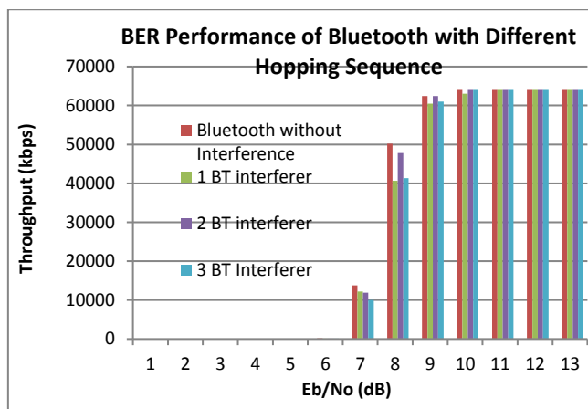
Fig. 6: Throughput Performance of Basic Bluetooth with Bluetooth Interference at different Hopping Frequency.
