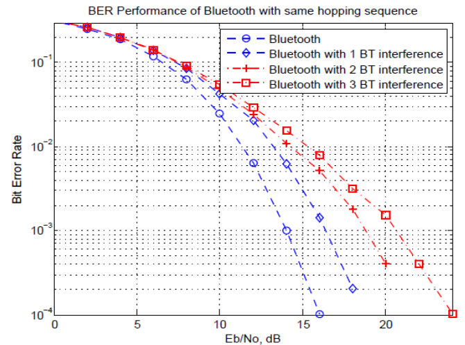
Fig. 2: BER Performance of Basic Bluetooth without Interference.
