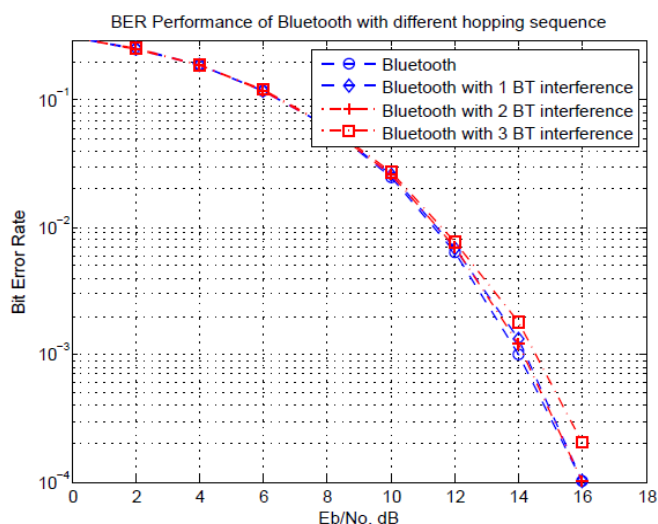
Fig. 3: BER Performance of Basic Bluetooth with Bluetooth Interferers.
