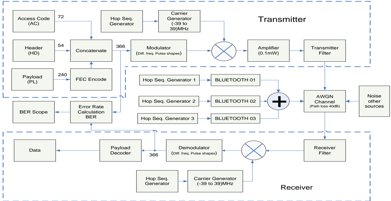
Fig. 1: Block Schematic of Bluetooth Transceiver.
