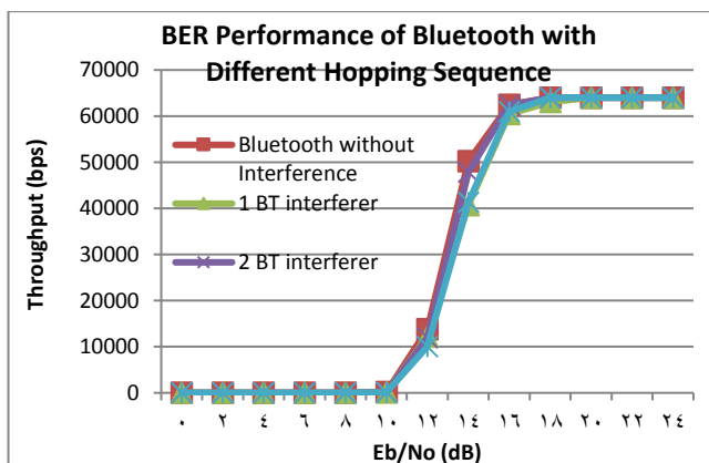
Fig. 5: Throughput Performance of Basic Bluetooth with Bluetooth Interference at different Hopping Frequency.
