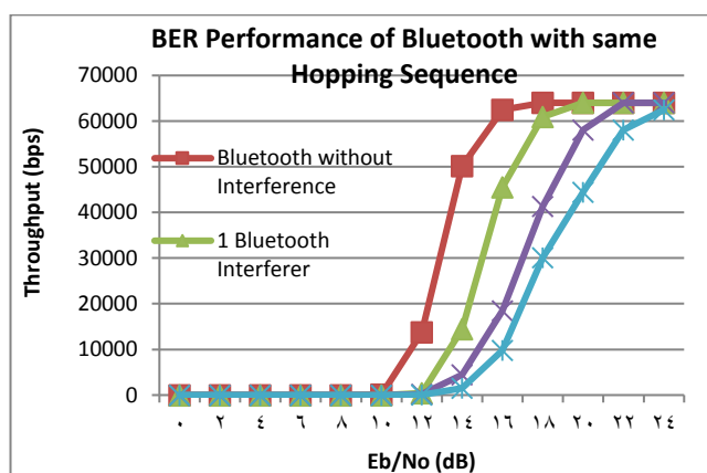
Fig. 4: Throughput Performance of Basic Bluetooth with Bluetooth Interference.
